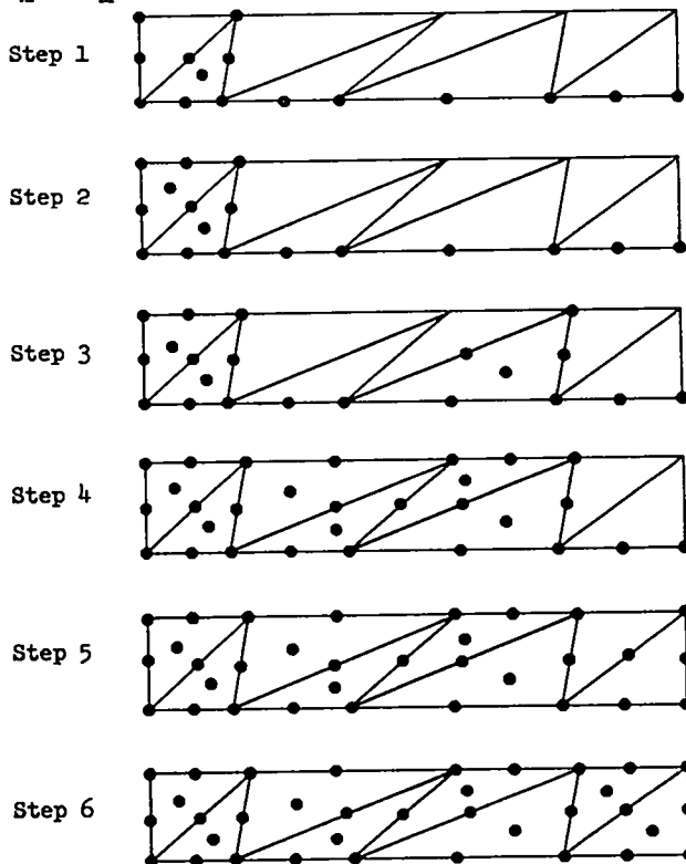
Fig. 10. A sample solution process on the band of triangles of Fig. 9. Dots represent known or determined fluxes.
