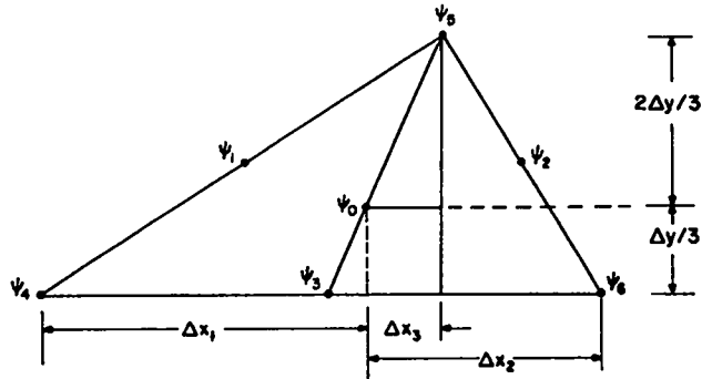
Fig. 17. Mesh definition for truncation error analysis.
